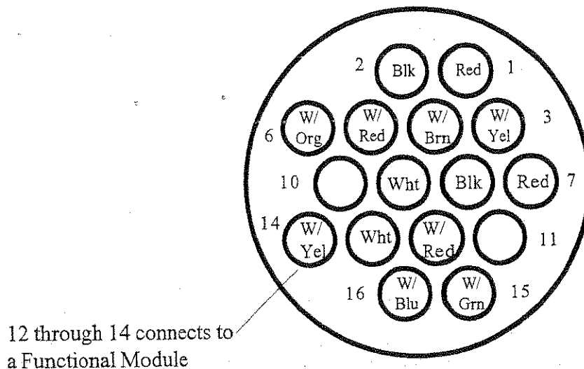
FP-5(L) Extension Cable Harness, Back View (wire side)
