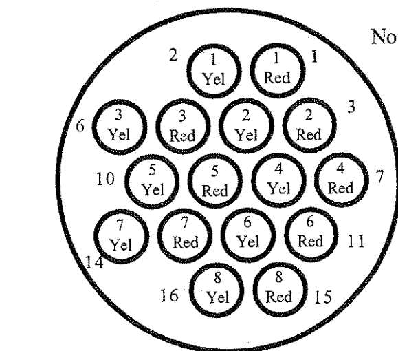
UBG Extension Cable Harness (Left or Right) Back View (wire side)
